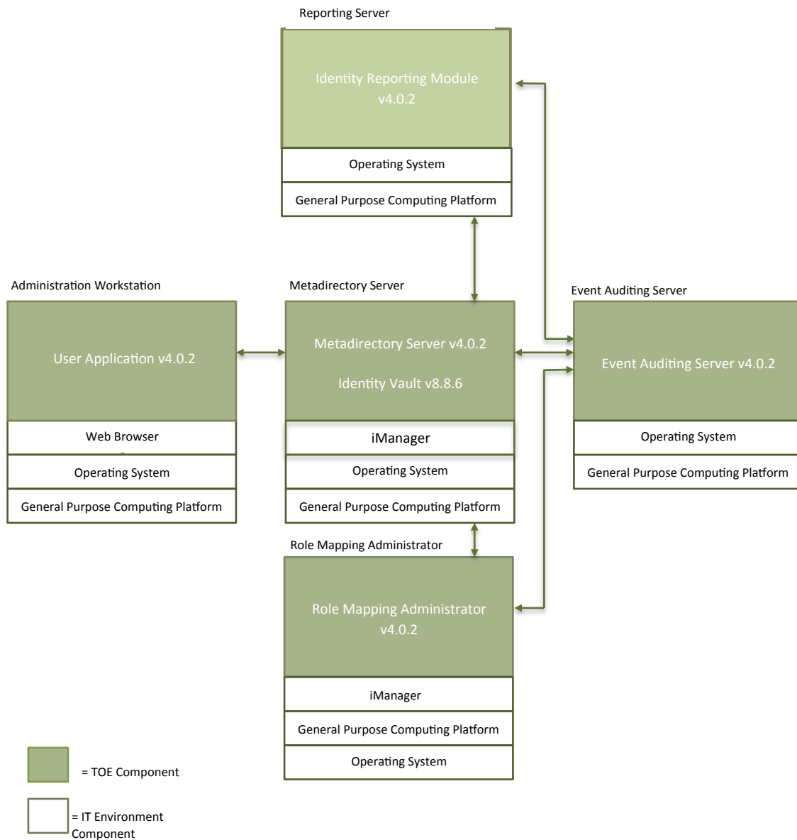
Figure 1 – TOE Deployment
